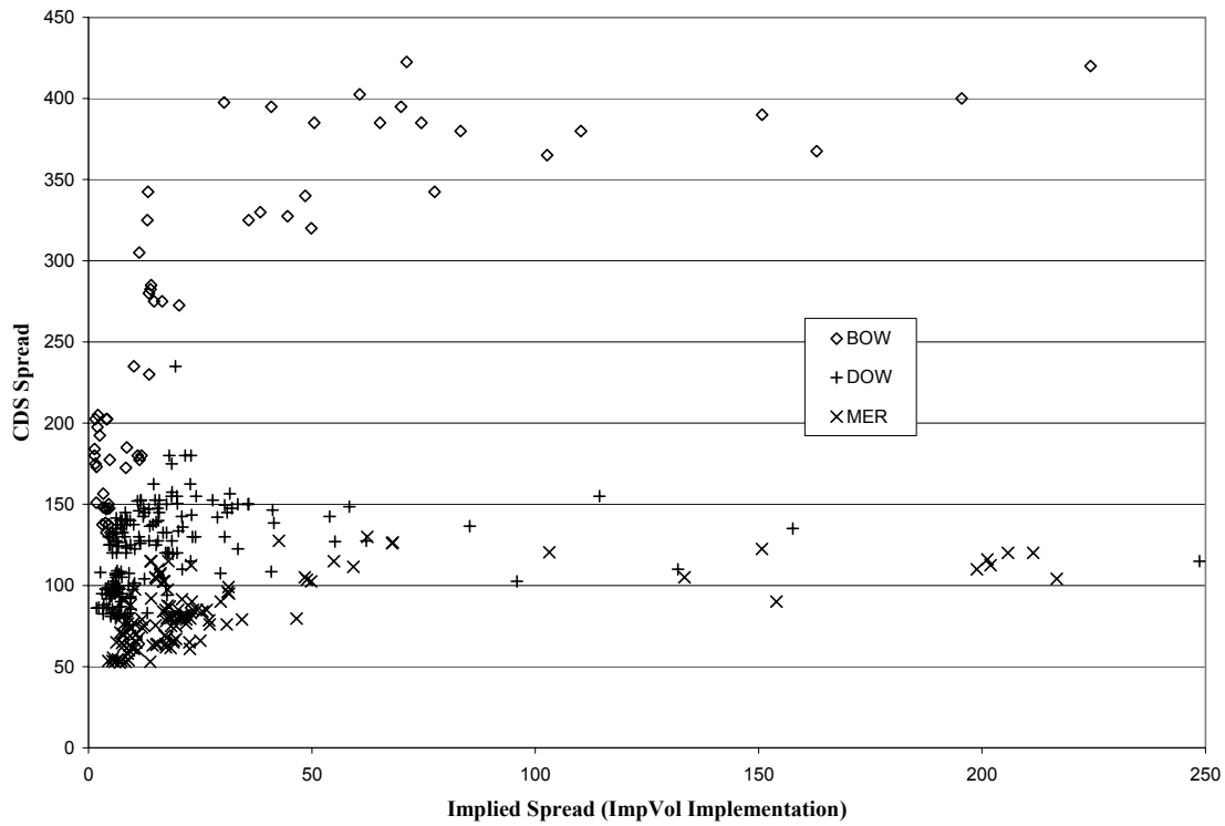
Figure 1: Relationship between CDS spread and implied spread for ImpVol Implementation of Merton's Model. The three companies are Merrill Lynch (MER), Bowater (BOW) and Dow Chemicals (DOW). The ImpVol implementation of Merton's model is the implementation we propose in equations (8) and (9).
